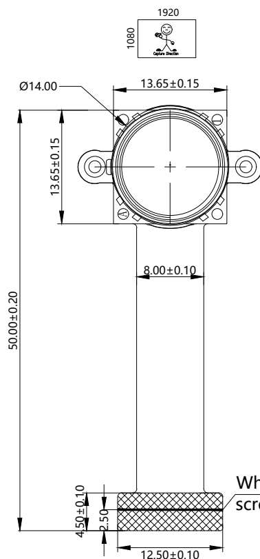
TOP VIEW
